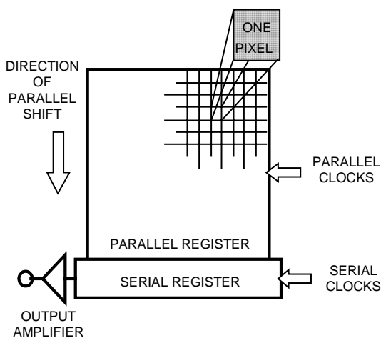
Figure 4 - Full-Frame Architecture
