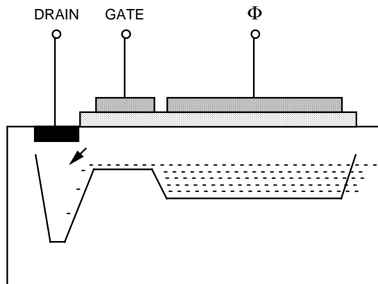
Figure 19 - Lateral Overflow Drain
