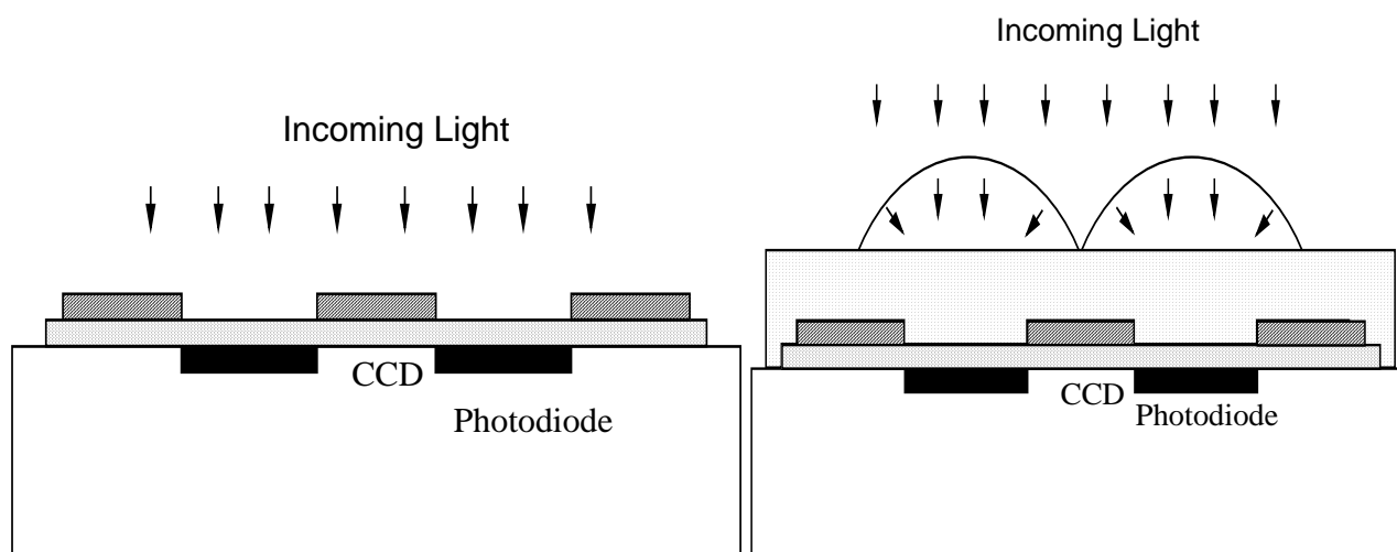
Figure 21 - Interline CCD Showing Photodiode and Non Sensitive CCD covered by a Light Shield
