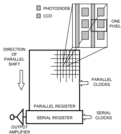
Figure 6 - Interline Architecture
