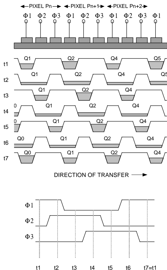
Figure 10 – Three-Phase CCD
