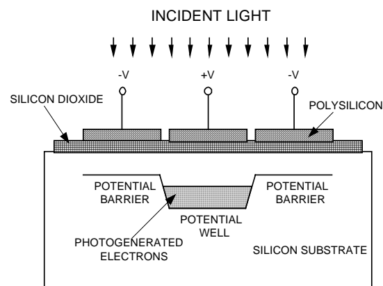
Figure 8 - Potential Well and Barriers
