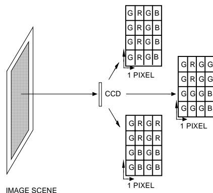
Figure 17 - Integral Color Filter Array Patterns
