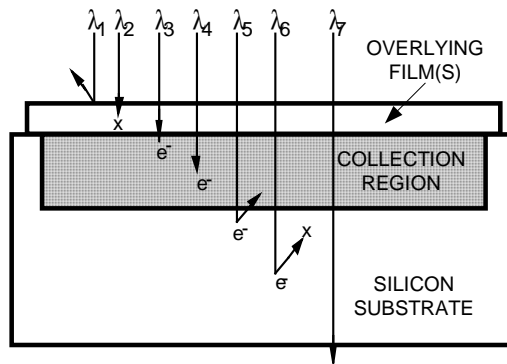
Figure 7 - Photon Interaction with Silicon
