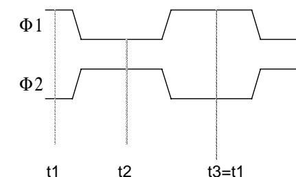
Figure 11 – Pseudo Two-Phase CCD
