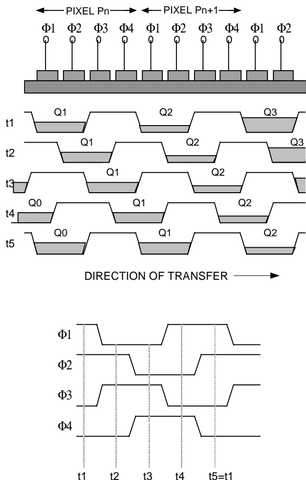
Figure 9 – Four-Phase CCD
