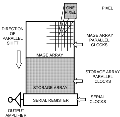
Figure 5 - Frame-Transfer Architecture
