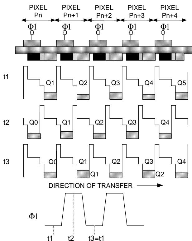
Figure 13 - Virtual Phase CCD
