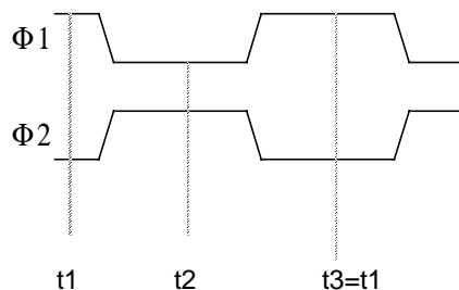
Figure 12 – True Two-Phase CCD
