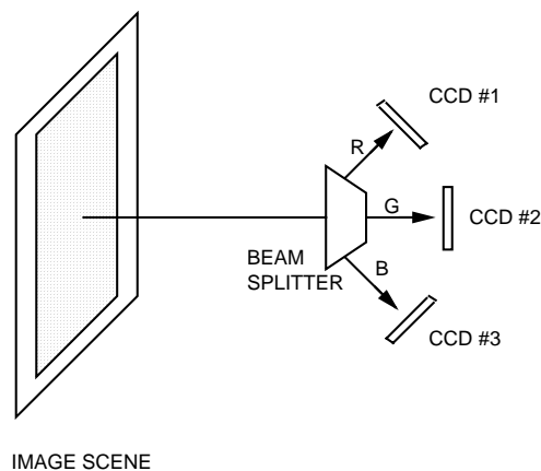
Figure 16 – Three-Chip Color Capture
